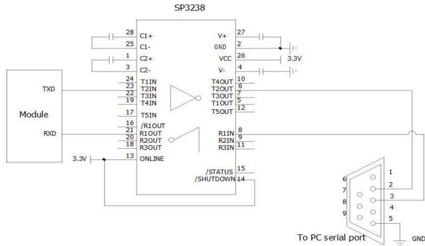
Figure 5: RS-232 Level Shift Circuit
