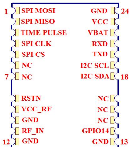
Figure 3: Pin Assignment
