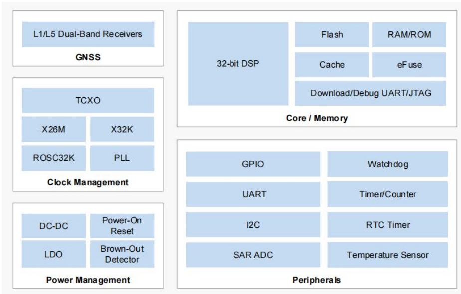
Figure 2: Block Diagram
