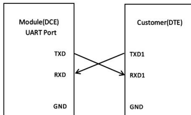
Figure 4:Serial Port Connection
