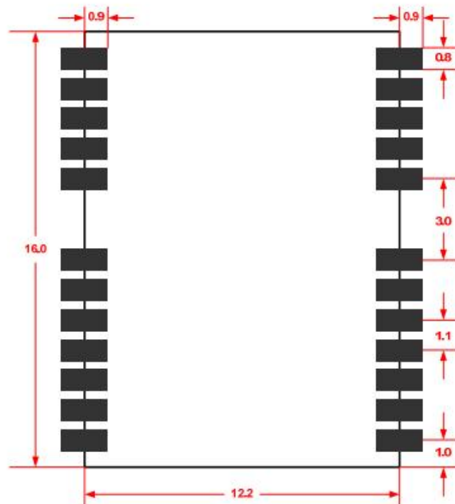
Figure 8: Reference Charging Size for PCB (unit: mm)
