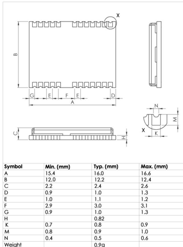
Figure 7: Mechanical Dimensions (Unit: mm)
