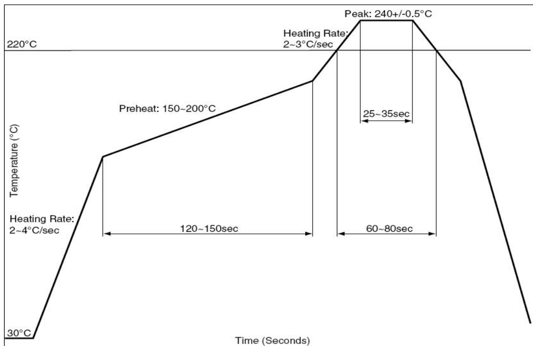
Figure 9: Recommended Reflow Soldering Thermal Profile
