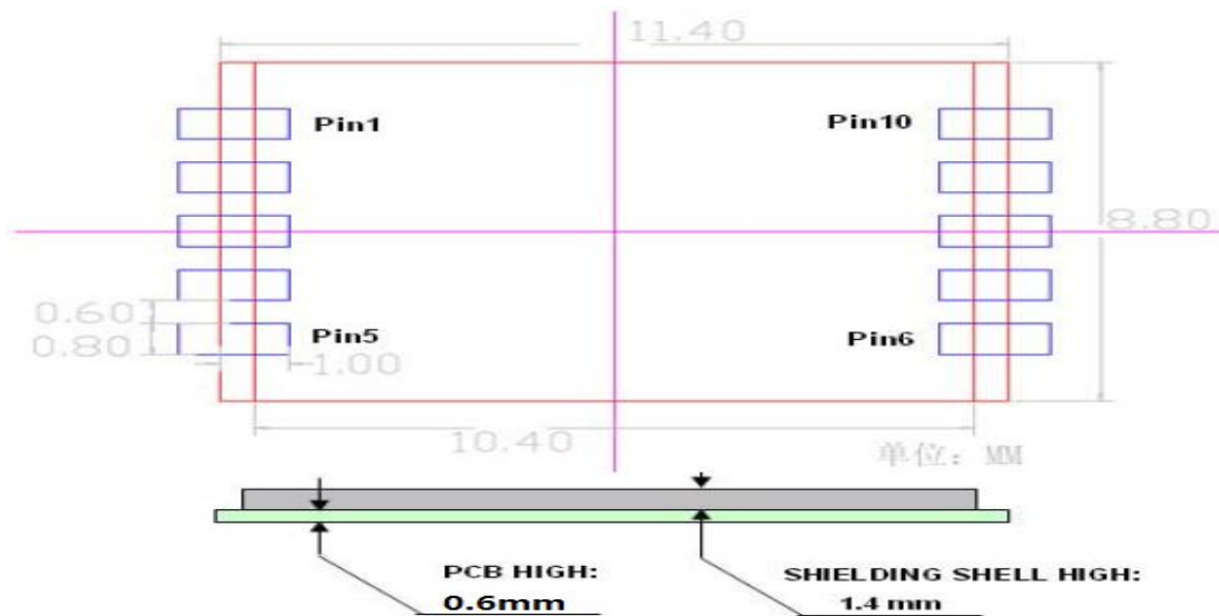
Figure 10: Top view Dimensions
