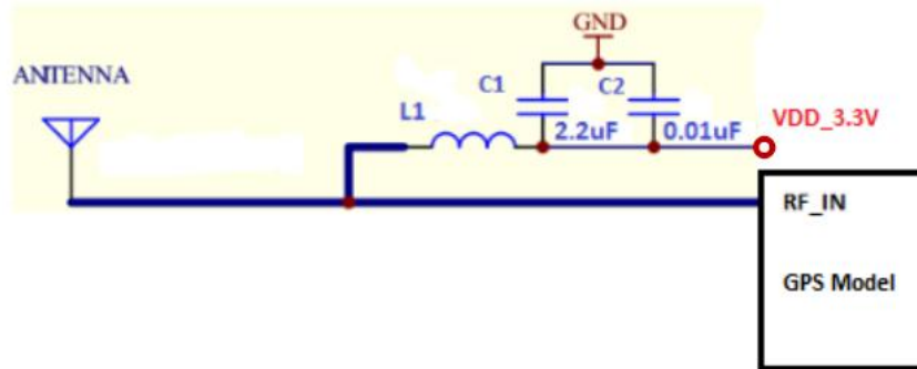
Figure 9: Reference Design for Active Antenna
