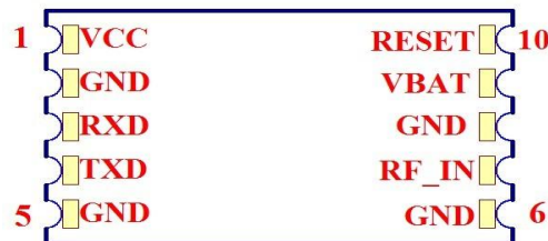
Figure 2: Pin Assignment
